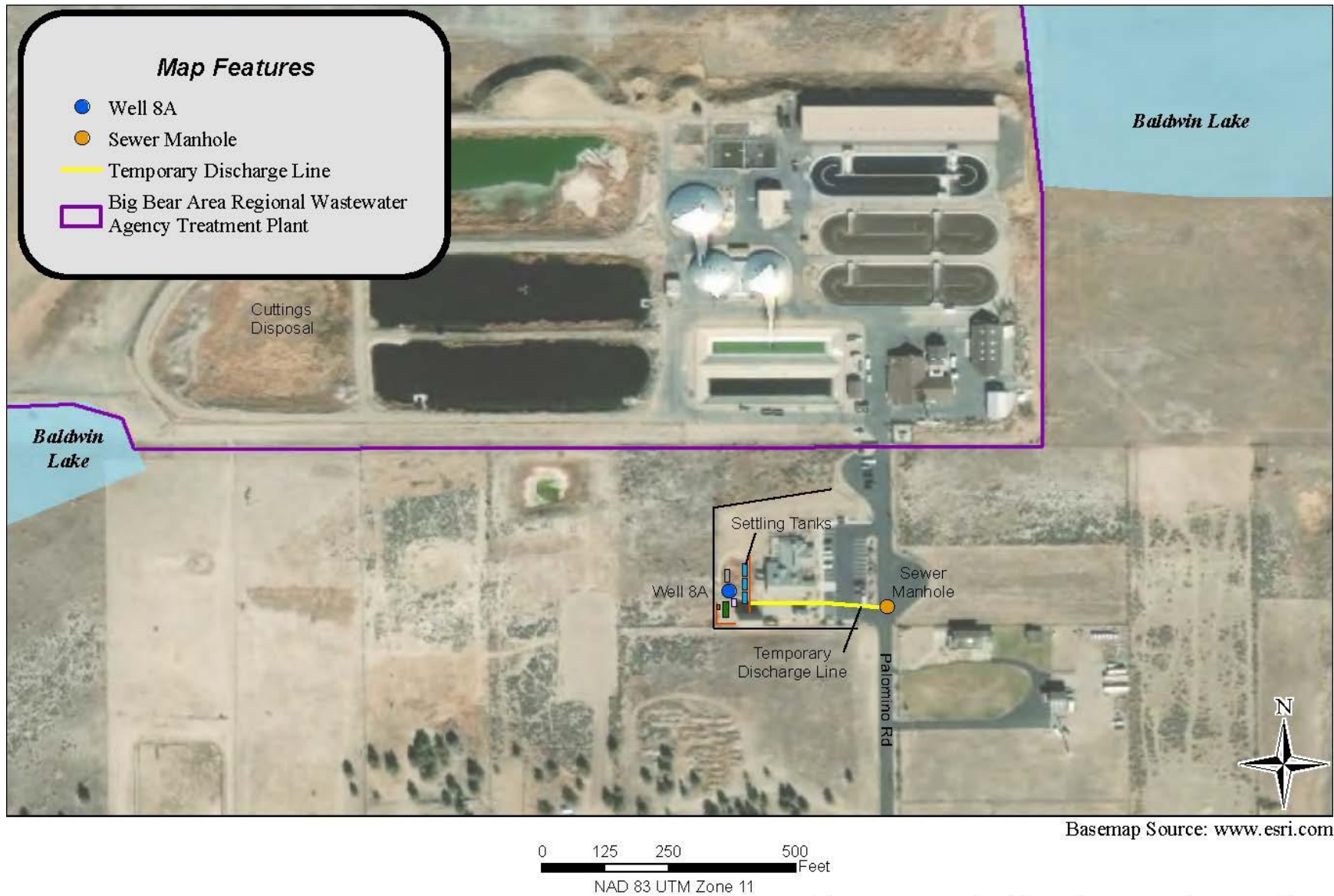
FIGURE 3b Aerial Photo of Specific Location of Well 8 and Proposed Well 8A
